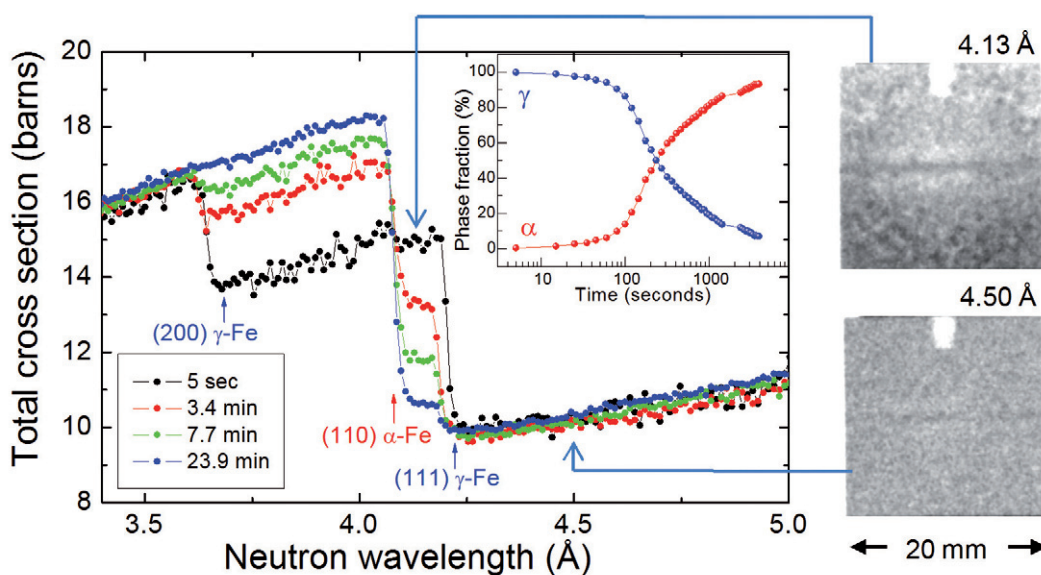
Fig. 5 Measured total neutron cross section of EN24 steel after austenization at 830 °C and kept in a furnace at 380 °C for the time specified. The inset shows the evolution of the volume fraction of the \alpha and \gamma phases as obtained by Rietveld analysis. The energy-selective radiographies on the right show another thermally treated steel sample, this time imaged at the two distinct neutron wavelengths \lambda given: The image on the top at \lambda = 4.13 Å (between the Bragg edges of \alpha -Fe and \gamma -Fe) shows residual austenite in dark due to its higher cross section. The image on the bottom (above the Bragg edge) is almost featureless because of the near equal cross sections for the both phases at \lambda = 4.50 Å. Reprinted with kind permission from Springer Science+Business Media 54 .
