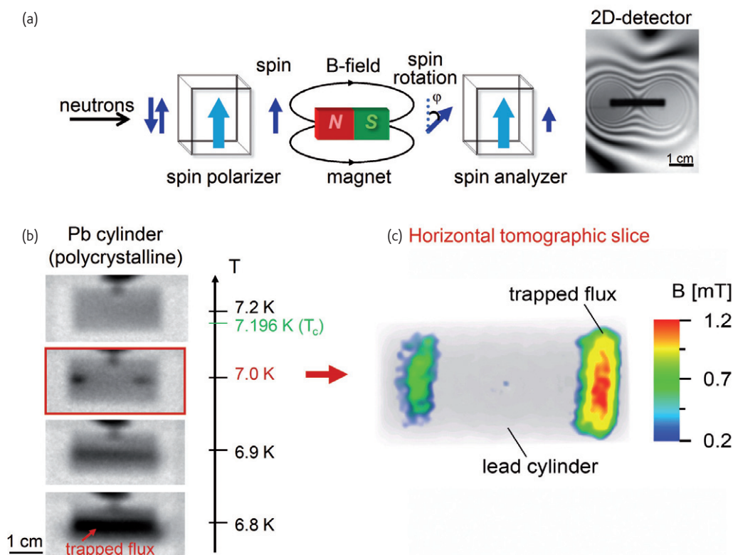
Fig. 9 (a) Incoming neutrons are first spin-polarized and then pass the magnetic field of a sample during which their spin vectors rotate by an angle, \phi , that is a sum of incremental rotations experienced along the neutron path. After this, they go through a polarization analyzer. Depending on the rotation angle, \phi , the transmission through the analyzer ranges from 0 to 1. This gives rise to a grey-scale image after measurement by the 2D detector. In the example given on the right, the field distribution around a magnet is visible. (b) The temperature dependence of the residual magnetic field trapped in a piece of superconducting lead is shown during step heating towards the transition temperature of superconductivity T_c . The inhomogeneous residual field decreases during heating and vanishes completely after T_c has been reached and superconductivity breaks down. (c) For a weak trapped residual field at T = 7.0 K, a tomographic investigation was performed by rotating the sample around the vertical axis. A quantitative reconstruction of the magnitude of magnetic field in a horizontal cross section through the centre of the tomogram can be obtained. Images first published in 83 . Reproduced with permission of the authors.
