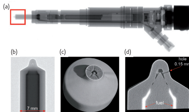
Fig. 2 Neutron imaging of a diesel injection nozzle. (a) Radiographic image of the entire injector; (b) high-resolution radiography of the nozzle; (c) and (d) tomographic reconstruction of the nozzle showing the fuel distribution in the nozzle channels. Reprinted from 9 . © 2007, with permission from Elsevier.
