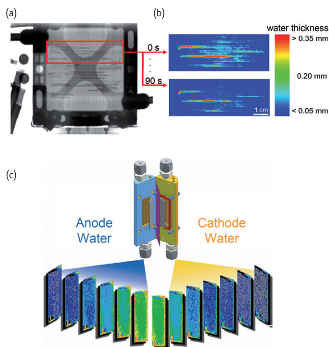
Fig. 3 (a) Neutron radiography of an operating fuel cell. Horizontal dark lines are caused by liquid water moving through the gas supply channels. (b) Water distribution in a PEM fuel cell directly after the cell supply has been switched from hydrogen to deuterium gas. \text{H}_2\text{O} has partially disappeared after 90 s since it has been exchanged by almost neutron-transparent \text{D}_2\text{O} . Reprinted with permission from 41 © 2008, American Institute of Physics. (c) Images of the water distribution obtained from tomographic measurement of a test fuel cell. The slices are 0.125 mm thick, yielding seven slices in each of the anode and cathode area. The peak of the water distribution is found in the anode of the cell. Reprinted from 44 with permission of DEStech Publications, Inc.
