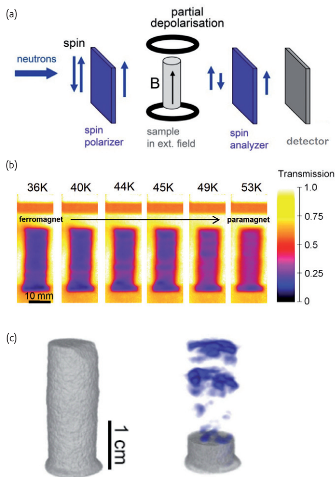
Fig. 10 (a) The principle of neutron depolarization imaging. (b) Temperature dependence of neutron depolarization of \text{Pd}_{1-x}\text{Ni}_x polycrystal which was grown with the Czochralski technique and has a nominal (global) Ni concentration of x = 3.14\% . \text{Pd}_{1-x}\text{Ni}_x is a weak itinerant ferromagnet with a strong dependence of the Curie-temperature, T_C , on the Ni concentration, x . Due to fluctuations of the Ni concentration within the sample, depolarization images show variations of the Curie temperature ranging from 36 K to 53 K over the sample. (c) A tomographic measurement was performed for another sample with x = 2.67 Ni. Here, Curie temperatures range from 5 K to 26 K. The measurement was performed at a constant temperature of T = 8 K. Paramagnetic regions of the sample are displayed in light grey, and ferromagnetic regions are blue. Reprinted from 93 with permission from IOP.
