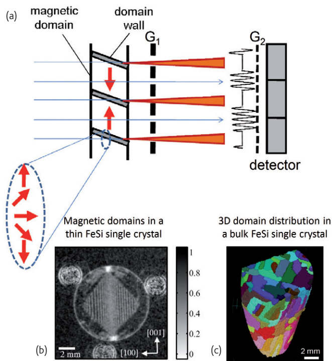
Fig. 8 (a) Refraction at domain walls results in a local decrease of the amplitude in the interference pattern. (b) Dark-field image of a thin (less than 1 mm) monocrystalline FeSi plate. The domain walls are visible as dark lines. Reprinted with permission from 87 . Copyright 2008, American Institute of Physics. (c) The magnetic domain structure of a bulk FeSi single crystal can be visualized in 3D by applying tomographic reconstruction algorithms to sets of 2D projections obtained at 100 different angles 89 . Colours have been introduced to distinguish between domains of different orientation.
