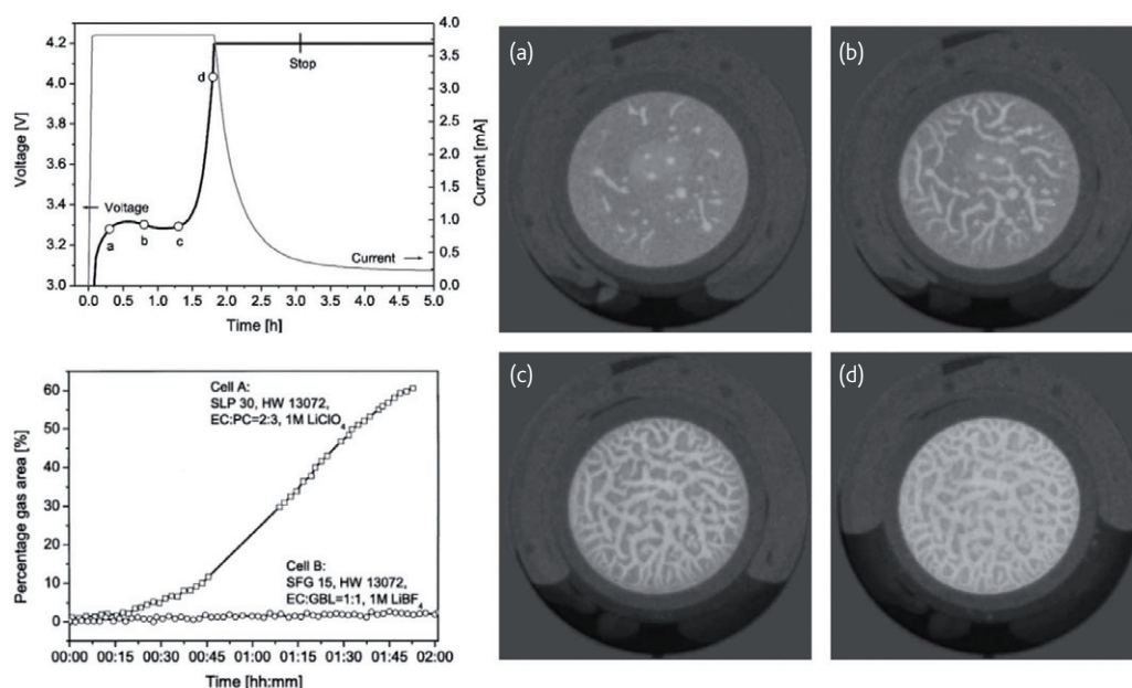
Fig. 4 Selected neutron radiographic images of a lithium ion cell assembled with a propylene-carbonate (PC) based electrolyte (cell A). The correlation with the state of charge is indicated in the top-left diagram (see letters a–d). The diagram on the bottom-left shows the percentage of the electrode area covered with gas bubbles for the two different electrolytes used: PC (cell A) and EC:GBL (cell B) as function of time. Reprinted from 47 . © 2004, with permission from Elsevier.
