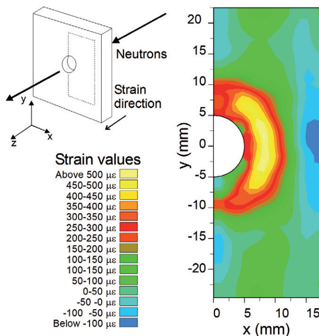
Fig. 6 Variation of the residual elastic strain in a cold-expanded hole in a 12 mm thick steel plate. The measured strains correspond to the through thickness average of the out-of-plane strains. Reprinted with kind permission from Springer Science+Business Media 54 .
