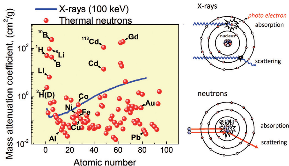
Fig. 1 Dependence of the mass attenuation coefficients of thermal neutrons (25 meV energy) and x-rays (100 keV energy) on the atomic number. Attenuation is a combined process of absorption (total removal of the particle) and scattering (deflection of the particle to outside the range of detection). The interaction of x-rays with the electrons of the electronic shell gives rise to a near-monotonic increase of the attenuation coefficient, while the nuclear interaction of neutrons with the different elements is not a regular function of the atomic number and also differs for different isotopes of the same element 1 . Reprinted from 16 with permission from Elsevier.
